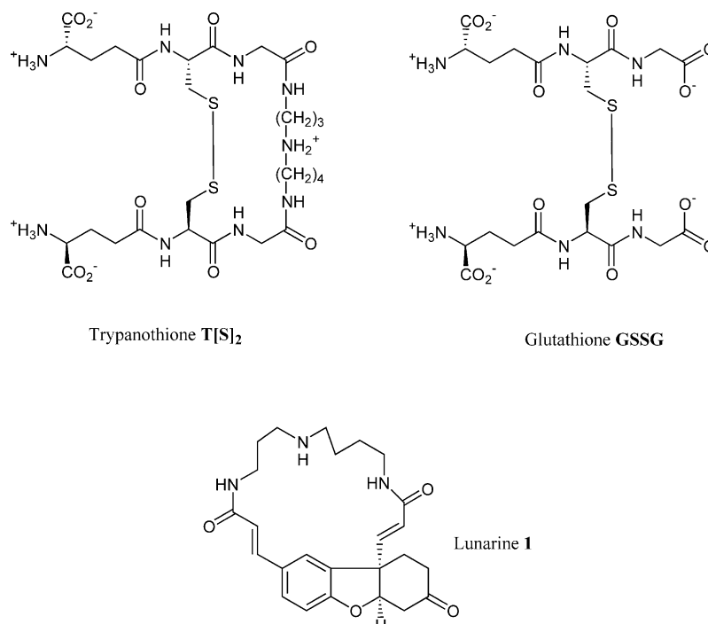
Figure 1. Native disulfide substrates for TryR ( T[S]_2 ) and GR ( GSSG ) and the time dependent inhibitor of TryR lunarine 1 .
