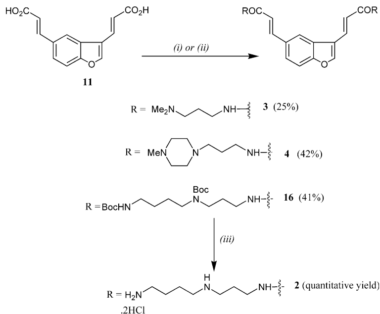
Scheme 4. Reagents and conditions: (i) \text{Ph}_2\text{P}(\text{O})\text{Cl} , \text{Et}_3\text{N} , DMF, -10^\circ\text{C} 1 h then add \text{RNH}_2 , 6 h; (ii) \text{C}_6\text{F}_5\text{OH} , EDCI, DMAP, DMF, 3 h then \text{RNH}_2 , \text{CH}_2\text{Cl}_2 , 2 h; (iii) 4 M HCl/dioxane, 1 h.
