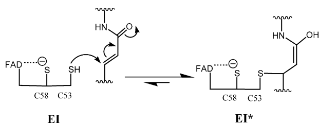
Figure 2. Proposed mechanism for time-dependent inactivation of TryR by the reversible formation of a covalent adduct between an active site thiol (C53) and one of the \alpha,\beta -unsaturated amide groups of lunarine 1 .
