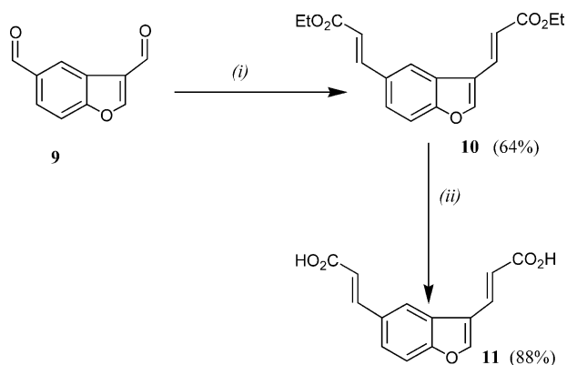
Scheme 2. Reagents and conditions: (i) \text{Ph}_3\text{P=CHCO}_2\text{Et} , \text{DMF} , reflux, 4 h; (ii) \text{LiOH} , \text{THF}/\text{H}_2\text{O}/\text{MeOH} , 4 h.
