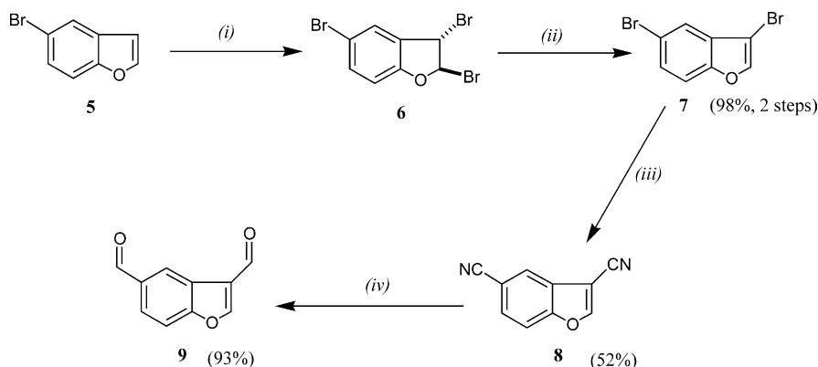
Scheme 1. Reagents and conditions: (i) \text{Br}_2 , \text{CH}_2\text{Cl}_2 , 40 min; (ii) \text{KOH} , \text{EtOH} , reflux, 15 min; (iii) \text{CuCN} , \text{DMF} , reflux, 16 h, then \text{FeCl}_3 , 1.5 M \text{HCl} , 70^\circ\text{C} , 30 min; (iv) \text{DIBAL} , \text{CH}_2\text{Cl}_2 , -15^\circ\text{C} , 3 min, then 1 M \text{HCl}_{(\text{aq})} , 0^\circ\text{C} .
