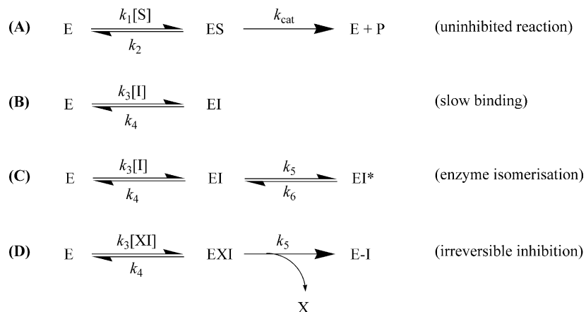
Figure 5. The basic mechanisms of time-dependent inhibition.
