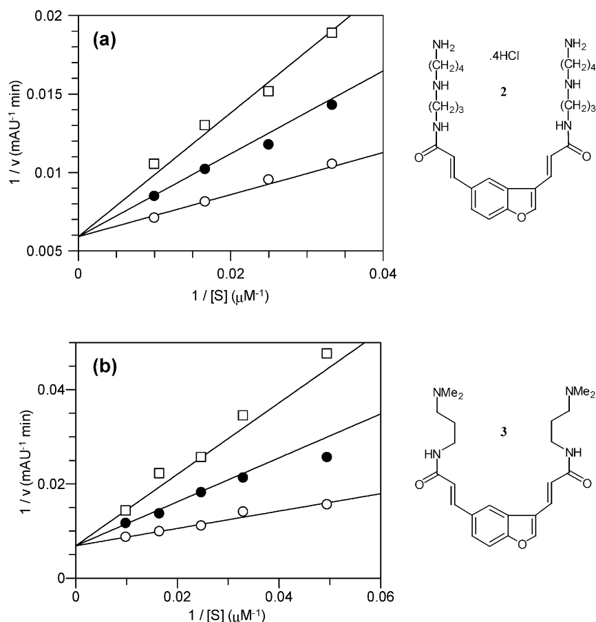
Figure 4. (a) Double reciprocal plots of initial rate against substrate concentration ( T[S]_2 ) in the presence of compound 2 at 0 μM (○); 100 μM (●); and 200 μM (□) concentrations. (b) Double reciprocal plots of initial rate against substrate concentration ( T[S]_2 ) in the presence of compound 3 at 0 μM (○); 293 μM (●); and 596 μM (□) concentrations.
