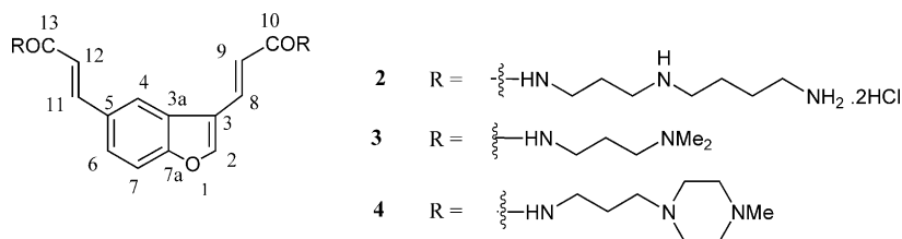
Figure 3. Structure of target compounds 2–4 .
