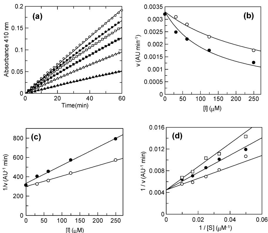
Figure 7. Inhibition of TryR by 1 . (a) Reduction in enzyme activity over time as a function of inhibitor concentration: no inhibitor (○); plus inhibitor: 31.25 μM (●); 62.5 μM (□); 125 μM (■); 250 μM (△); 500 μM. (b) Re-plot of variation in v_i (○) and v_s (●) with respect to concentration of 1 . These data were fitted to eqs 2 and 3 to derive values for K_i and K_i^* , respectively (Table 1). (c) Variation of the reciprocal of v_i (○) and v_s (●) as a function of concentration of 1 . (d) Double reciprocal plot of v_i against substrate concentration in the presence of no inhibitor (○); plus inhibitor: 100 μM (●); 200 μM (□) to demonstrate the competitive nature of inhibition by 1 .
