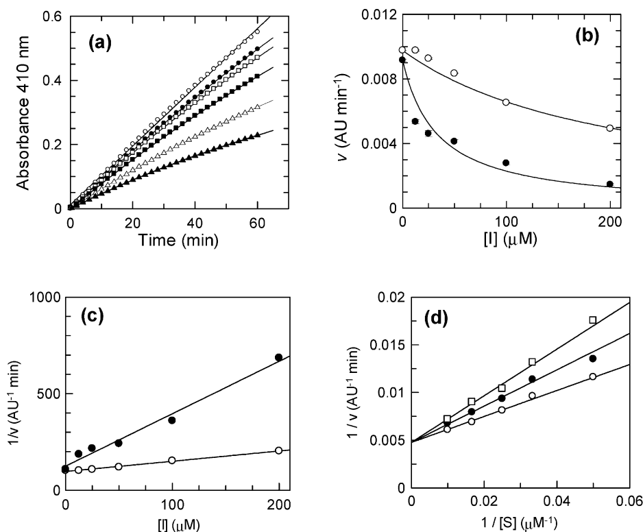
Figure 6. Inhibition of TryR by 4 . (a) Reduction in enzyme activity over time as a function of inhibitor concentration: no inhibitor (○); plus inhibitor: 12.5 μM (●); 25 μM (□); 50 μM (■); 100 μM (△); 200 μM (▲). (b) Re-plot of variation in v_i (○) and v_s (●) with respect to concentration of 4 . These data were fitted to equations (2) and (3) to derive values for K_i and K_i^* , respectively (Table 1). (c) Variation of the reciprocal of v_i (○) and v_s (●) as a function of concentration of 4 . (d) Double reciprocal plot of v_i against substrate concentration in the presence of no inhibitor (○); plus inhibitor: 100 μM (●); 200 μM (□) to demonstrate the competitive nature of inhibition by 4 .
